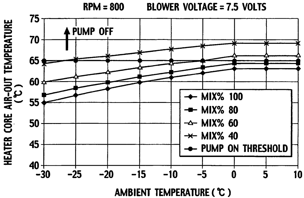
FIG.5 HEATER CORE AIR-OUT TEMP. PERFORMANCE (85°C HWI)
